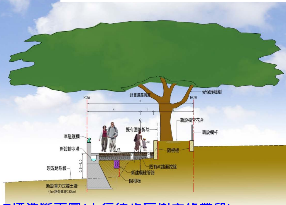
OK+065.6 ~ OK+103.7標準斷面圖(人行徒步區樹穴綠帶段)
