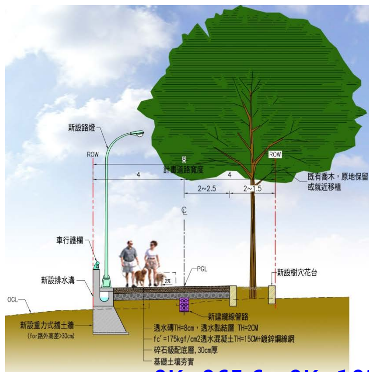
OK+065.6 ~ OK+103.7標準斷面圖(人行徒步區樹穴綠帶段)
